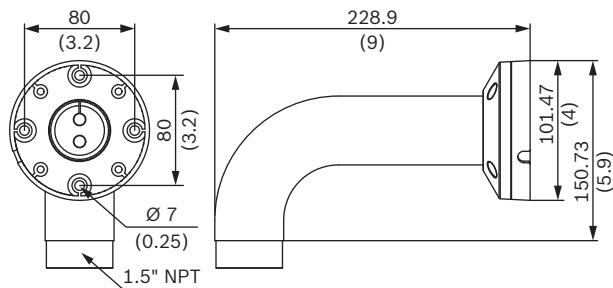
NDA-U-WMT Pendant wall mount Dimensions in mm (inch)
